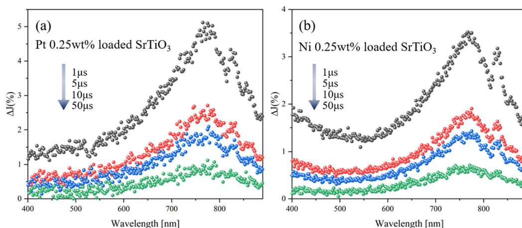
Fig. 4 (a) Transient absorption spectra of Pt 0.25 wt% loaded \text{SrTiO}_3 particles and (b) Ni 0.25 wt% \text{SrTiO}_3 particles irradiated by a UV (355 nm) pulsed laser under \text{N}_2 gas. The pump energy was 1.3 \text{ mJ cm}^{-2} , and the repetition rate was 10 Hz.
