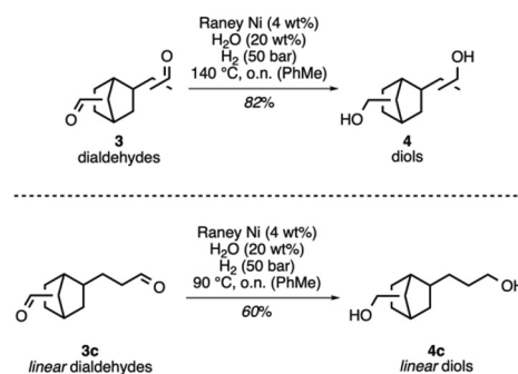
Scheme 3 Optimized hydrogenation strategy for the scale-up synthesis of diols 4 and linear diols 4c .
