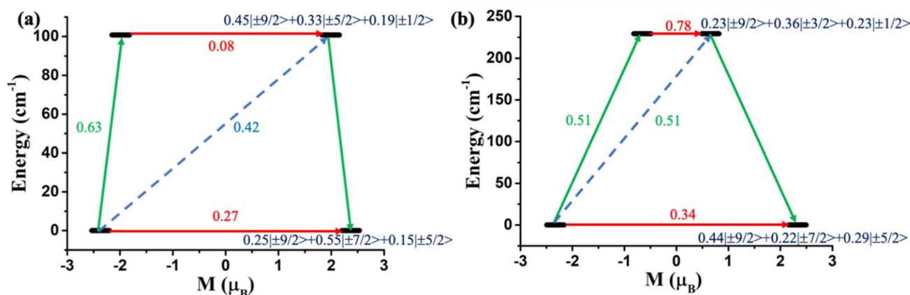
Fig. 7 The mechanism of magnetization relaxation of (a) [U(Tp^{Me_2})_2(THF)_2] (7) and (b) [U(Tp^{Me_2})_2CH_2Ph] (9). The red arrows denote the QTM via the ground state and TA-QTM via the first excited state. The sky-dotted arrow represents the Orbach process. The green arrows indicate the most possible pathway of magnetisation relaxation.
