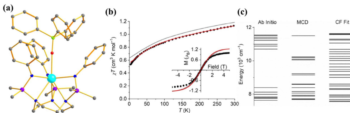
Fig. 8 (a) The molecular structure of the complex [U(\{SiMe_2NPh\}_3-tacn)(OPPh_3)] (12). Colour code: U (cyan), N (blue), Si (violet), P (green) and C (grey). Hydrogens of complexes are omitted for clarity. (b) Experimental vs. computed temperature-dependent magnetic susceptibility of 12 (experiment: circles, ab initio : grey, fitted: red). The inset shows the M vs. H comparison of complex 12. (c) The experimental vs. computed crystal field splitting energy level of complex 12. Reprinted with permission from ref. 6 and reproduced with permission from John Wiley and Sons.
