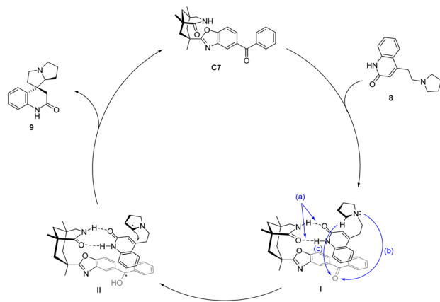
Fig. 3 Mechanism of asymmetric conjugate addition of \alpha -aminoalkyl and ketene catalyzed by xanthone C7.
