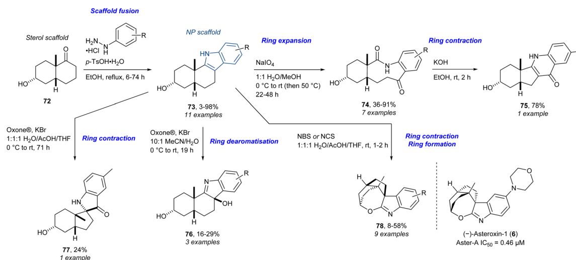
Scheme 6 Synthesis of sterol-inspired compounds and identification of Aster-A inhibitor (–)-asteroxin-1 ( 6 ). 35 Oxone ^\circ = \text{KHSO}_5 \cdot 0.5\text{KHSO}_4 \cdot 0.5\text{K}_2\text{SO}_4 , NBS = N -bromosuccinimide, NCS = N -chlorosuccinimide.
