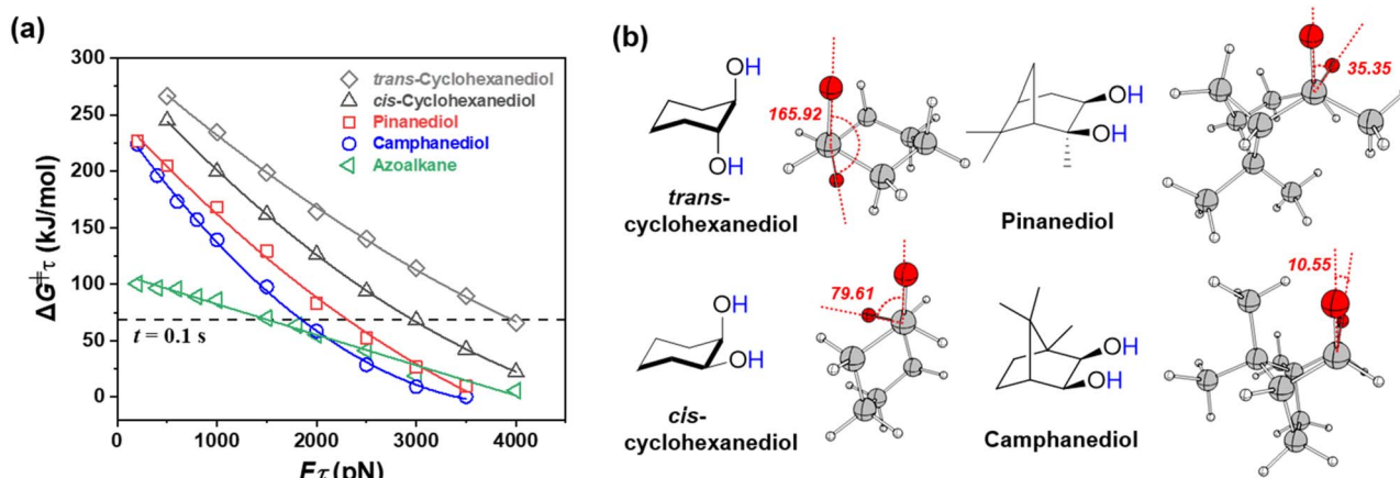
Fig. 3 (a) Computed \Delta G^\ddagger_\tau - F_\tau graph at the UB3LYP-D3/6-311G(d,p)//UB3LYP-D3/6-311G(d,p) level of theory for the homolytic cleavage of the C–C bond in a series of vicinal diols. The x-axis represents the level of simulated tensile force, while the y-axis indicates the force-coupled free energy barrier for C–C bond cleavage. The \Delta G^\ddagger_\tau - F_\tau curve of a conventional mechanophore, azoalkane, is also included as a reference. (b) Optimised structures of the force-coupled transition states under F_\tau = 2000 pN, highlighting the presence of a “node” in camphanediol, characterised by an O–C–C–O dihedral angle of 10.55^\circ .
