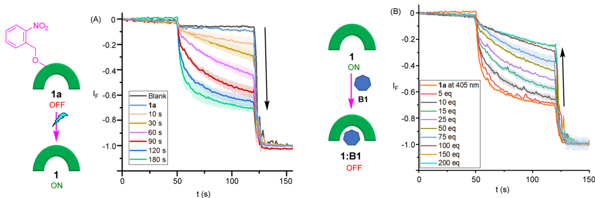
Fig. 5 (A) Ion transport activities across POPC-LUVs of lucigenin after photo-irradiating 1a at 405 nm light using an LED (1 W) and (B) treating 1a with light for 5 minutes followed by the addition of barbiturate ligand B1 .
