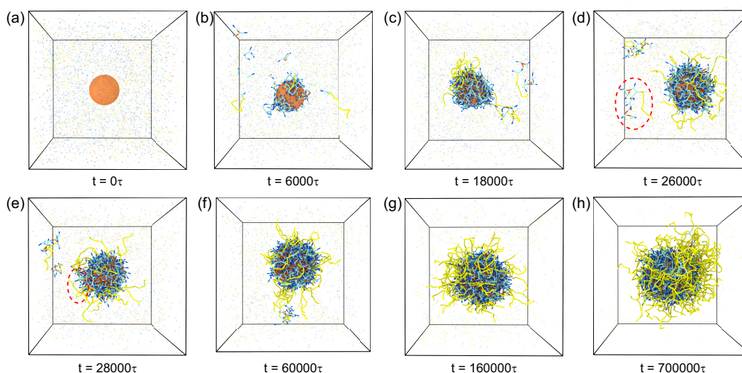
Figure 4 Time-resolved morphological evolution of n(sphere) assemblies during polymerization. Snapshots illustrate the growth process under optimized stoichiometric conditions with fixed CE_{10} hydrophilic chain concentration (0.00519 mol/L). Reaction simulation parameters were maintained at \alpha_{OA} = 6.0 and P_r = 0.005 throughout the process. Temporal progression is indicated below each snapshot. For visual clarity, solvent beads are omitted. Color scheme is the same as in Figure 1: central nanosphere (gold), crosslinkers (pink), adsorption beads (dark blue), polymerization beads (light blue), and hydrophilic chains (yellow).
