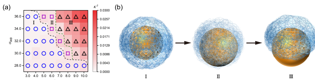
Figure 3 Morphological characteristics in n(sphere) assemblies. (a) Systematic variation of adsorption capacity ( \alpha_{OA} : 3.0 - 10.0) and hydrophobicity ( \alpha_{WB} : 28.0 - 36.0) modulates nanocapsule anisotropy ( \kappa^2 ), with outlined thresholds for morphological transitions. (b) Schematics for delineating three characteristic morphological regimes: I) Fully encapsulated structures, II) Distorted encapsulations, and III) Partially exposed structures. All systems were prepared at the same stoichiometry under optimized parameters ( P_r = 0.005 ). Schematic representations emphasize core-shell architecture (gold: central nanosphere, light blue: polymer network) with peripheral chains omitted for clarity.
