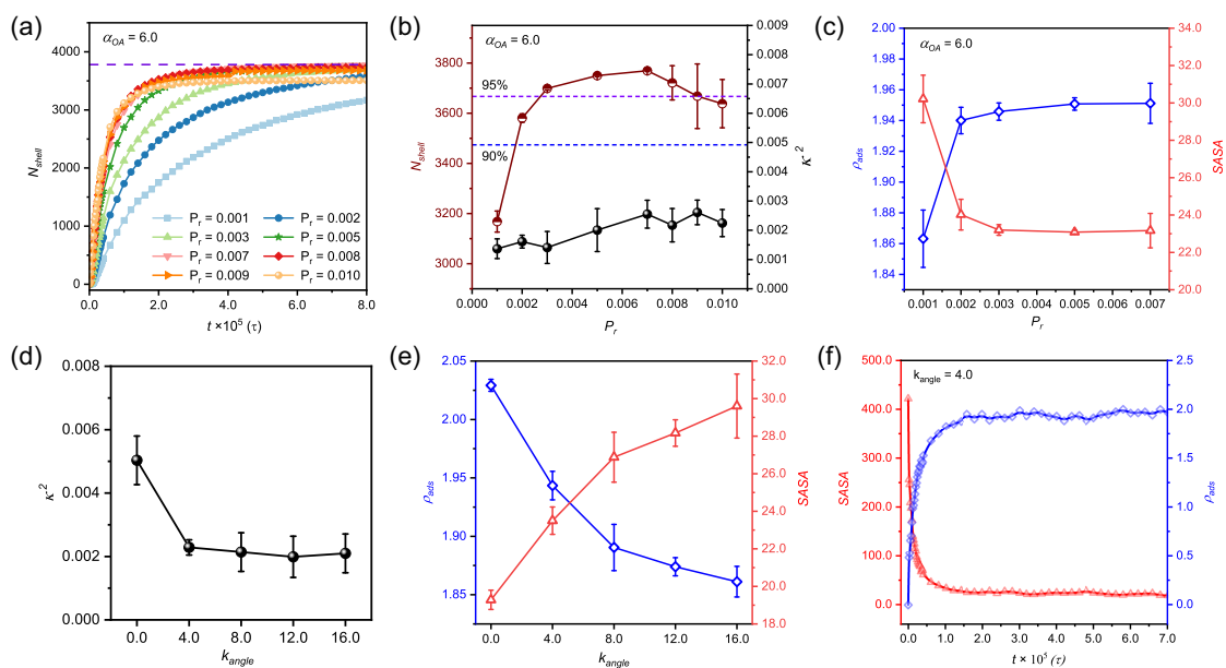
Figure 2 Influence of reaction probability and chain rigidity on structural parameters and morphological characteristics. (a) Temporal evolution of the number of beads in polymer shell ( N_{shell} ) at varying reaction probabilities ( P_r ) with fixed adsorption strength ( \alpha_{OA} = 6.0 ). (b) Correlation between stabilized N_{shell} values and corresponding relative shape anisotropy ( \kappa^2 ) across different P_r values at \alpha_{OA} = 6.0 , with dashed lines indicating distinct monomer utilization efficiency. (c) Dual-parameter analysis of SASA and \kappa^2 as functions of reaction probability at \alpha_{OA} = 6.0 . (d) Dependence of \kappa^2 on chain rigidity ( k_{angle} ) under optimized conditions ( \alpha_{OA} = 6.0 , P_r = 0.005 ). (e) Quantitative assessment of adsorption density ( \rho_{ads} ) and SASA with various chain rigidities. (f) Time evolution of SASA and \rho_{ads} at an intermediate chain rigidity ( k_{angle} = 4.0 ). The molar ratios of monomers, crosslinkers, and initiators in panels (a) to (f) are 75:14:1, namely n_{(M)} : n_{(C)} : n_{(I)} = 75:14:1 .
