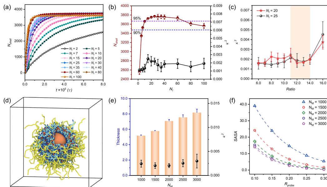
Figure 5 Composition-dependent morphological evolution of n(sphere) assemblies. (a) Temporal evolution of the number of beads in polymer shell ( N_{shell} ) at varying initiator concentrations ( N_I ) under fixed conditions ( n_C: n_I = 14:1 , N_M = 1500 ). (b) Dependence of relative shape anisotropy ( \kappa^2 ) and N_{shell} on different initiator concentrations. (c) Crosslinker concentration-dependent relative shape anisotropy ( \kappa^2 ) at optimal initiator concentrations ( N_I = 20, 25 ), expressed versus n_C: n_I ratio. (d) Snapshot of n(sphere) morphology at N_M = 2000 , revealing internal structural organization. (e) Monomer concentration effects on shell thickness and relative shape anisotropy ( \kappa^2 ). (f) Solvent accessibility (SASA) as a function of monomer concentration, with probe size = 0.1 (symbols: simulation data; dashed line: fitted curve). In the simulation snapshot, solvent is not shown for clarity and the color settings are the same as those in Figure 1. All simulations were conducted under standardized conditions ( \alpha_{OA} = 6.0 , P_r = 0.005 ).
