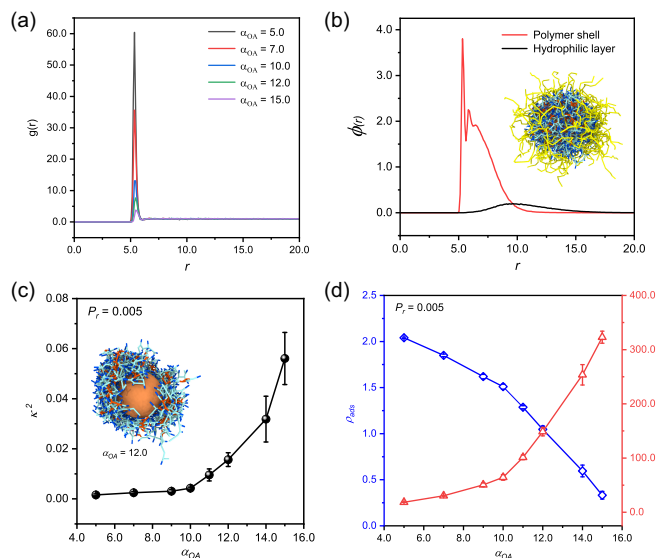
Figure 1 Structural characterization and adsorption-dependent properties of stabilized n(sphere) assemblies. (a) Radial distribution function (RDF) profiles of monomer (A-B) at varying adsorption capacities ( \alpha_{OA} ) in the pre-polymerization state. (b) A radial density profile of well-defined n(sphere) structures under optimal conditions ( \alpha_{OA} = 6.0 , P_r = 0.005 ), with the corresponding conformations inserted. (c) Correlation between relative shape anisotropy ( \kappa^2 ) and adsorption interaction strength ( \alpha_{OA} ) at constant reaction probability ( P_r = 0.005 ). The inbuilt image corresponds to the asymmetric n(sphere) conformation at \alpha_{OA} = 12.0 . The outer hydrophilic chain ( E_{10} ) has been omitted for clarity of the image. (d) Dual-parameter analysis showing the interdependence of solvent accessible surface area (SASA) and monomer adsorption density ( \rho_{ads} ) as functions of \alpha_{OA} . All systems were maintained at a fixed stoichiometric ratio of n_{(M)} : n_{(C)} : n_{(I)} = 75:14:1 (monomer: crosslinker: initiator). Visual representations employ the following color: central sphere (O, gold), crosslinkers (C-C, pink), monomer adsorbable beads (A, dark blue), polymerizable beads (B, light blue), and hydrophilic chains ( E_{10} , yellow). Solvent molecules are omitted from visualization for clarity.
