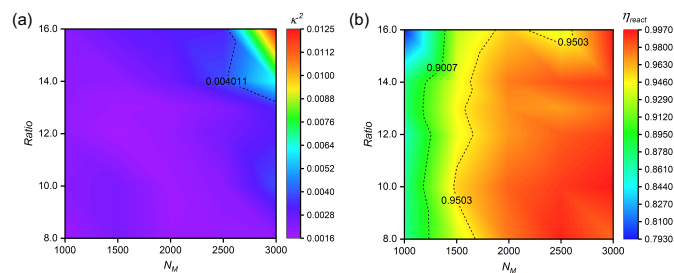
Figure 6 Concentration-dependent structural optimization and reaction efficiency. (a) Correlation between reactant concentrations and relative shape anisotropy ( \kappa^2 ) of n(sphere) assemblies. (b) Reaction efficiency ( \eta_{react} ) as a function of monomer concentration at optimized stoichiometry. All systems maintain fixed n_M: n_I = 75:1 , with crosslinker content expressed as n_C: n_I ratio. Simulations were conducted under standardized conditions ( \alpha_{OA} = 6.0 , P_r = 0.005 ). Data points represent averaged values from five independent replicates.
