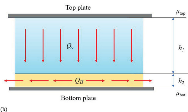
Fig. 5 (a) Fluid outflow from the sample visualized by colored liquid. A fibrin gel at a concentration of 15\ \text{mg ml}^{-1} was polymerized with a blue stained buffer. After compression the colored fluid leaves the sample only from the bottom over a period of minutes. (b) Schematic representation of fluid flow in our compressed gel samples. The flow in the upper layer (height h_1 ) is directed downward, while the flow in the lower layer (height h_2 ) is radial. The chemical potential at the middle of the top plate is denoted by \mu_{\text{top}} and that at the middle of the bottom plate \mu_{\text{bot}} . The lower layer thickness h_2 is significantly smaller than the upper layer thickness h_1 ( h_2 \ll h_1 ). These two layers are not to be confused with densified and rarefied phases that are formed under compression.
