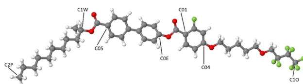
Fig. 4 Snapshot of the initial simulation box with molecules arranged in a SmA phase, containing four layers. A few selected molecules are highlighted for clarity.
