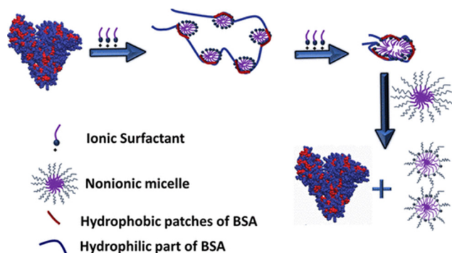
Fig. 4 Schematic showing the unfolding of BSA protein in the presence of ionic ( C_{12}TAB ; n = 10, 12, 14 and 16 ) surfactants and then refolding upon further addition of nonionic ( C_{12}E_{10} ) surfactants at pH 7. All tested cationic surfactants induce BSA unfolding, where the denatured state is depicted as a beads-on-a-string configuration, consistent with a random flight model. Upon subsequent addition of the nonionic surfactant, C_{12}E_{10} , mixed micelles are formed, which effectively sequester the ionic surfactant away from the protein. Reproduced from ref. 12 with permission from the American Chemical Society, copyright 2018.
