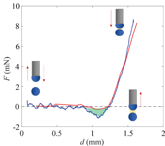
Fig. 5 Force–displacement plot at contact force F_M = 10 mN, relative humidity RH = 80\% , t_c = 1 s and retraction speed v_r = 0.006 mm s −1 . The approach curve is represented by — , and retraction curve by — . The green part represents the area under the F – d plot and hence the total dissipation in the loss of contact. Here, d means the distance by which the upper sphere is lowered respective to the initial position.
