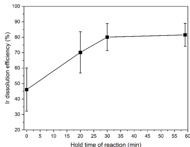
Fig. 2 Kinetic model of the extraction of Ir into solution at various holding times. T = 139 °C, [Cl^-] = 1.6 M, [H_2O_2] = 3\% v/v, S/L = 0.25 g L^{-1} . The measurements were conducted three times, and the average results are presented, with error bars representing the standard deviation of the three replicates.
