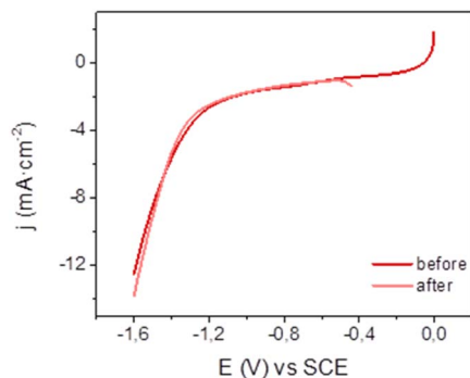
Fig. 7 Linear sweep voltammetry of Mn@Terpy-COF|NT ([Mn] total = 850 \mu\text{mol cm}^{-2} ) on CP at 10 \text{mV s}^{-1} before and after CPE at -1.3 \text{ V} vs. SCE in water \text{K}_2\text{SO}_4/\text{K}_2\text{B}_4\text{O}_7 under \text{CO}_2 .
