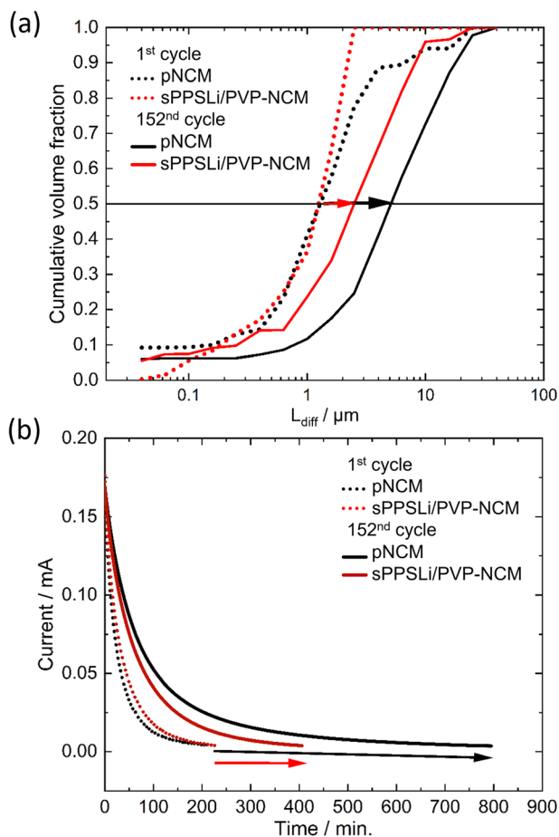
Fig. 7 (a) L_{\text{diff}} obtained using the EIS-PSD model for \text{LiIn}^{\text{SEB}^{\text{pNCM}}} and \text{LiIn}^{\text{SEB}^{\text{sPPSLi/PVP-NCM}}} in the 1st and 152nd cycles. The Warburg impedance is fitted through the EIS-PSD model to yield the cumulative volume fraction of particle size of different L_{\text{diff}} . (b) The chronoamperometry measurement shows the duration required for the current to drop below 2% of the initial charging current, which is proportional to L_{\text{diff}} .
