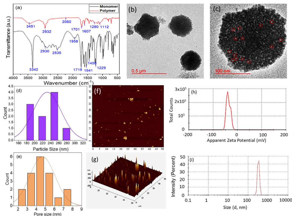
Fig. 1 (a) FTIR spectra showing the absorption band for the Gly monomers and polymers, (b) and (c) HRTEM images of GlyNPs at 0.5 \mu m and at 100 nm scale; (d) particle size distribution calculated from HRTEM images taking 100 particles, (e) pore size distribution of the particles calculated from (c), (f) AFM topography 2D image and (g) 3D AFM image; (h) plot for zeta potential results obtained from DLS and (i) hydrodynamic diameter of the polymeric particles calculated from a Zetasizer. Particles are of size 180–20 nm. The pore size obtained to be avg. 4–5 nm in diameter (highlighted with a red circle). (c) Zeta potential obtained to be -35.6 mV. Scale for the AFM image is in \mu m.
