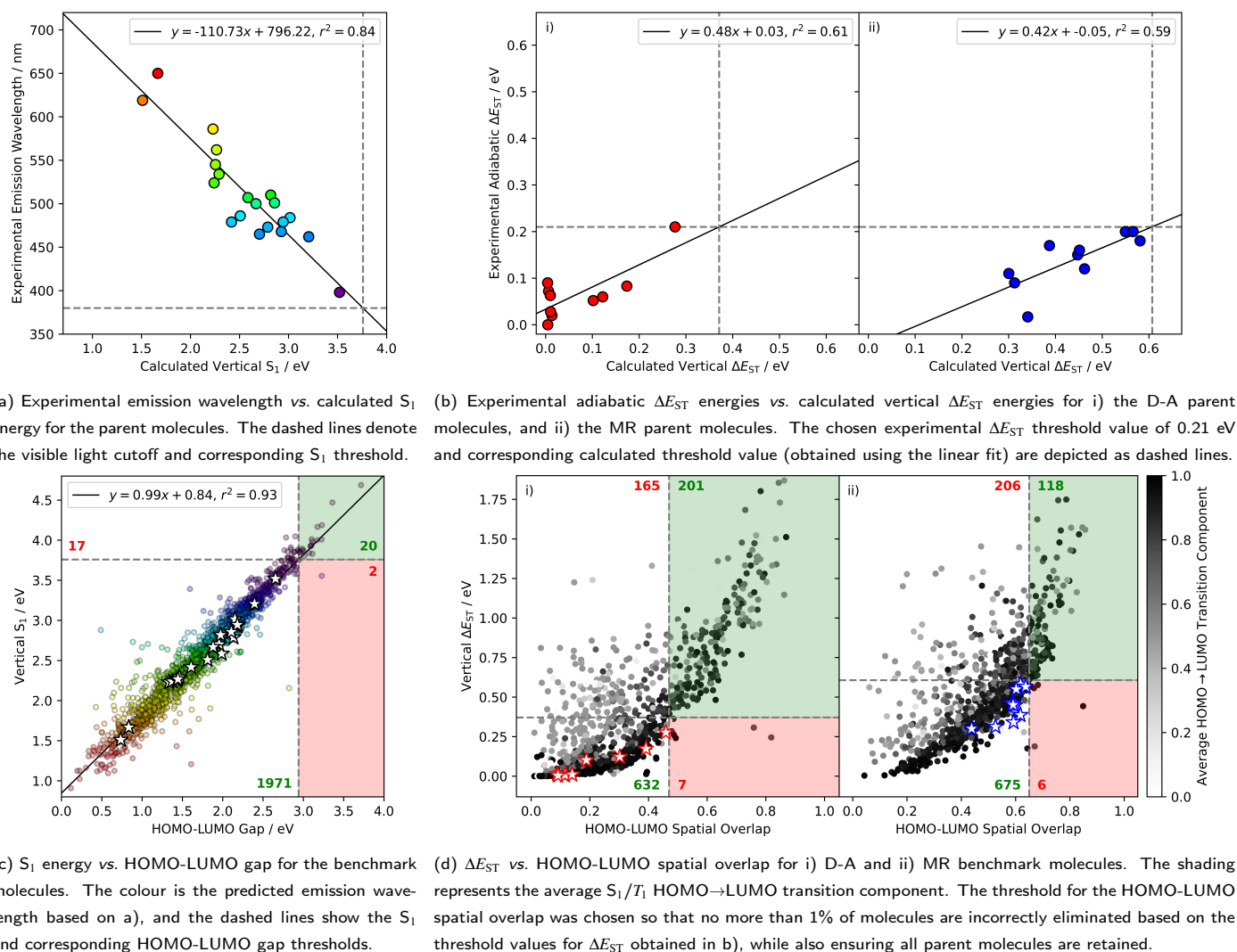
Fig. 3 Benchmarking plots for determining the screening thresholds for HOMO-LUMO gaps and overlaps. The green (red) shaded regions in c) and d) show molecules which are correctly (wrongly) eliminated following the HOMO-LUMO calculation. The corresponding numbers of molecules are written in green (red), as are those which are correctly (needlessly) retained in the unshaded areas. For c) and d) parent molecules are highlighted using the ★ symbol. S_1 , \Delta E_{ST} and HOMO→LUMO transition components were calculated using TDDFT at the B3LYP/6-31G* level on the DFT-optimised geometries, while HOMO-LUMO gaps and overlaps were calculated using PBE and a wavelet basis on the xTB-optimised geometries. Experimental values are from Refs 9,12,70–87 ; the \Delta E_{ST} value for DHPZ-2TRZ is recorded as “nearly zero”, and so was approximated to zero.
