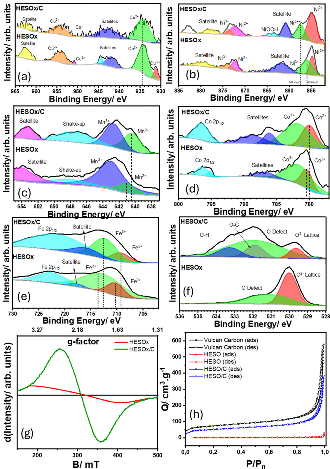
Fig. 3 (a)–(e) shows the deconvoluted 2P XPS spectra of the five metals in both HESOX and HESOX/C. (f) shows the oxygen 1S XPS spectra (g) EPR spectra of HESOX and HESOX/C. (h) N 2 absorption–desorption curves.
