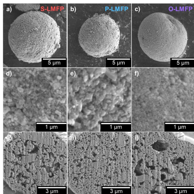
Fig. 3 SEM images of LMFP samples synthesized with (a,d,g) LMFO, (b,e,h) \text{NH}_4\text{Fe}_{0.5}\text{Mn}_{0.5}\text{PO}_4 , and (c,f,i) separate oxide precursors. Spray dried secondary particles (a-c) in their entirety and (d-f) zoomed into the surface of the secondary particle to investigate the primary particles. (g-i) FIB-SEM images of the cross-section of the secondary particles.
