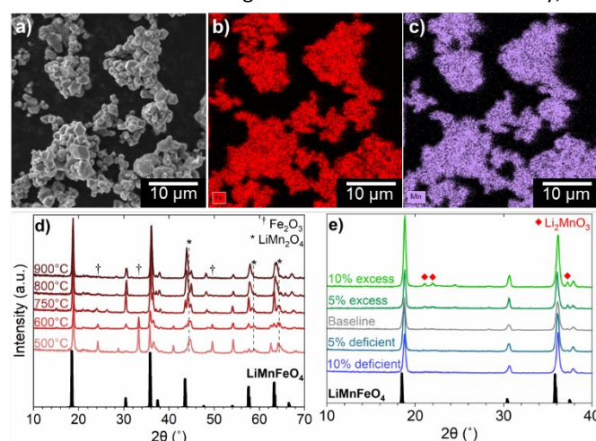
Fig. 1 (a) SEM image of LMFO spinel precursor with EDS mapping of (b) Fe and (c) Mn. XRD patterns of LMFO (d) heated from 500 to 900 °C and (e) with adjusted Li amounts, from 10% deficient Li to 10% excess Li based on molar ratios. JCPDS #04-008-1660, #00-035-0782, #00-039-1346, and #00-027-1252 are used to identify the phases as, respectively, LMFO, LiMn 2 O 4 , Fe 2 O 3 , and Li 2 MnO 3 .
