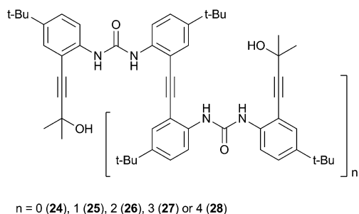
Jeong and co-workers have reported a series of diphenylureas 24–28 that form foldamer complexes with chloride and sulfate. 18 The solution phase sulfate binding properties were investigated by 1 H NMR titration in 20% and 40% CD 3 OH–DMSO- d 6 . In both cases the sulfate binding strength was found to increase with increasing chain length from 24–28 by approximately 4 orders of magnitude. In contrast, chloride binding studies in 15% CD 3 OH–acetone- d 6 indicated that the binding strength reached a plateau after receptor 26 ( K_a = 1340 \text{ M}^{-1} ). The authors attributed this difference to the greater hydrogen bond acceptor ability of sulfate, with the tetrahedral array of oxygen atoms allowing the formation of up to 12 hydrogen bonds, whereas chloride can be coordinatively saturated by fewer urea groups. The crystal structure of 25 ·(Bu 4 N) 2 SO 4 confirmed the encapsulation of a single SO 4 2− anion in a 1 : 1 foldamer complex with each anion coordinated by four hydrogen bonds from two urea groups, and a further two hydrogen bonds from peripheral OH groups (Fig. 5).
