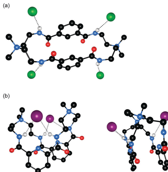
Fig. 2 (a) Crystal structure of 9 2+ ·2Cl − ·2.66H 2 O (b) two views on the crystal structure of 10 2+ ·2I − ·2H 2 O. Hydrogen bonds are shown as dashed lines; solvent molecules and non-coordinating hydrogens are omitted for clarity; chloride is represented in green spacefill; iodide in purple spacefill and the receptors are shown in ball-and-stick.
