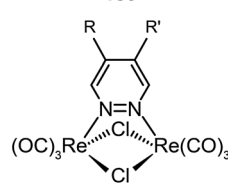
182: R = \text{H} , R' = \text{n-hexyl}
