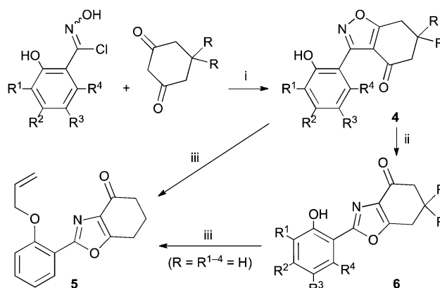
Scheme 2 Synthesis and rearrangement of 3-aryltetrahydrobenzoxoxazoles 4 . Reagents: (i), NaOi-Pr, i-PrOH; (ii), Cs 2 CO 3 , THF reflux; (iii), H 2 C=CHCH 2 Br, Cs 2 CO 3 , THF reflux.
