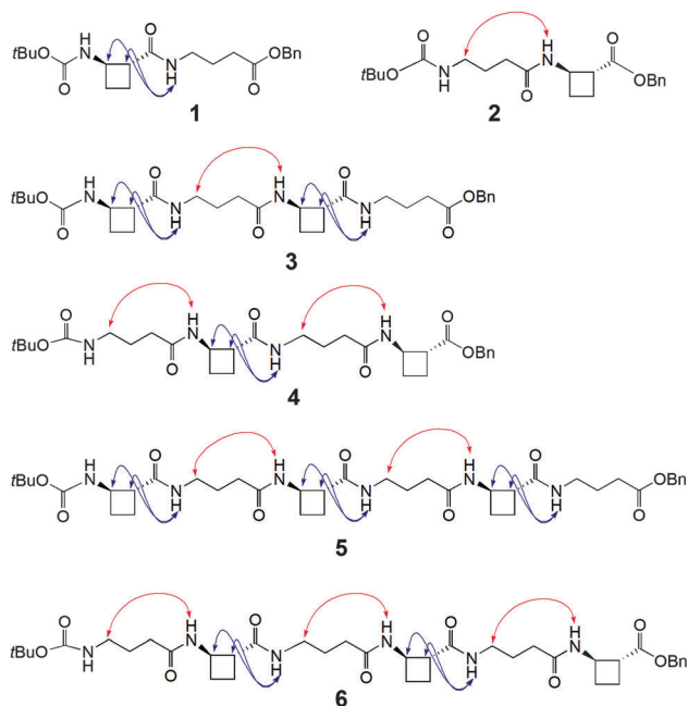
Fig. 1 Molecular structures of \beta/\gamma -peptides 1–6 and ROESY correlations observed in \text{CDCl}_3 (10 mM).
