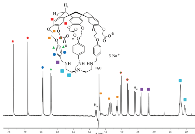
Fig. 1 ^1\text{H} NMR spectrum (500.1 MHz, \text{D}_2\text{O} , 298 K, \text{pD} \approx 7 ) of hemicyptophane 3 .
