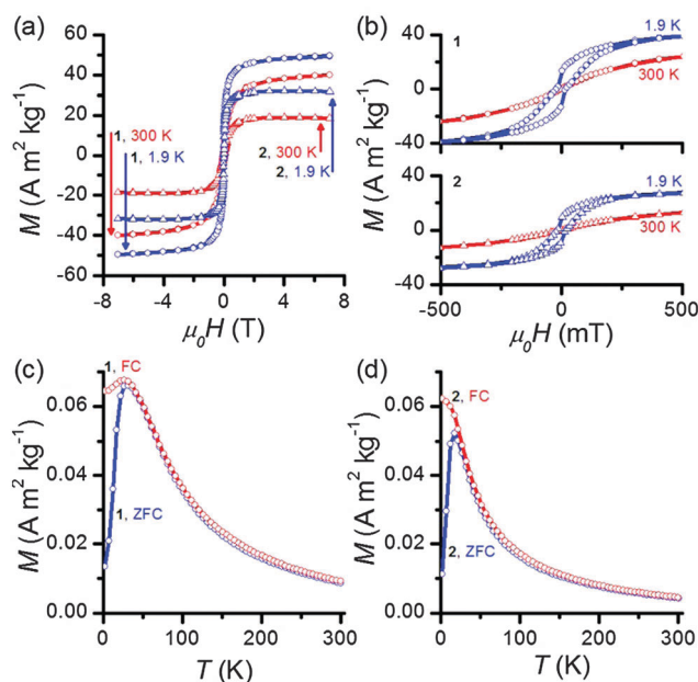
Fig. 2 Magnetic properties of 1 and 2 . (a) M vs. H loops to 7 T at 1.9 and 300 K, (b) showing the low-field region and the emergence of hysteresis at low temperature for both 1 and 2 . (c and d) Field-cooled (FC) and zero-field-cooled (ZFC) measurements showing temperature-dependent magnetization under 10 mT. For 1 , the blocking temperature ( T_B ) is 32 K, indicated by the peak of the ZFC curve (c), and for 2 (d) T_B = 17 K. Based on the shape of the FC-ZFC plots, the particle size distribution of both 1 and 2 appears narrow.
