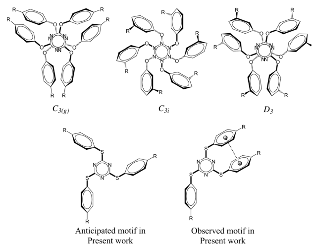
Chart 1 Piedfort units of tris-aryloxytriazines (TArOTz) with 3-fold symmetry ( \text{C}_{3(g)} , \text{C}_{3i} , and D_3 ) 17–21,23–25 and the motif anticipated and observed in the present work for tris-arylthiotriazines (TArTTz).
