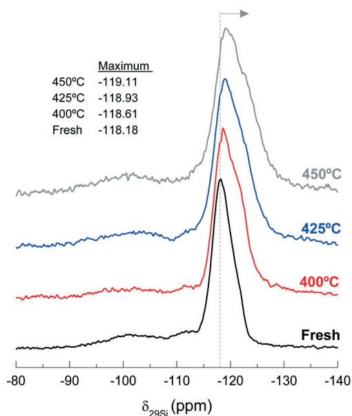
Fig. 11 Effect of reaction temperature on the peak position of 29 Si NMR spectra, –118.18 ppm, of the fresh and used catalysts during 255 min time on stream.
