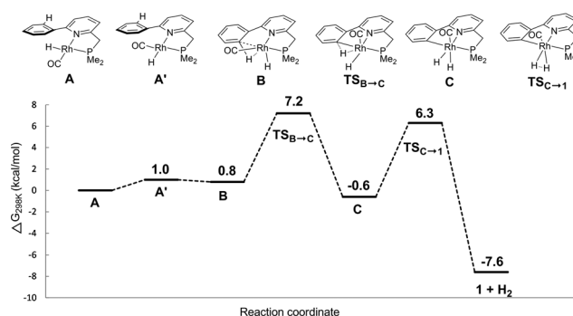
Fig. 3 DFT (BP86, def2-TZVP, disp3) calculated free energy profile ( \Delta G_{298\text{K}}^0 in kcal mol −1 ) of dihydrogen formation from hydride intermediate A Me , with methyl instead of tert -butyl groups.
