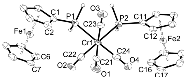
Fig. 2 Molecular structure of cis -[Cr(CO) 4 (PH 2 Fc) 2 ] ( 2a ). The hydrogen atoms of the ferrocenyl moieties are omitted for clarity. Ellipsoids drawn at 50% probability. Only one of the two symmetry-independent molecules is shown.
