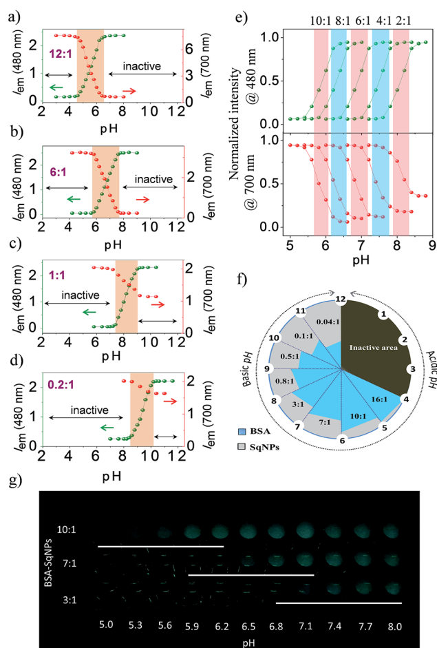
Fig. 3 (a)–(e) Fluorescence intensity of BSA–SqNP hybrid nanosensors in the 480 ( \lambda_{\text{ex}}@380 \text{ nm} ) and 700 nm ( \lambda_{\text{ex}}@640 \text{ nm} ) region at different pH conditions. The active pH range for different ratios is indicated by the shadow color. (f) A pictorial representation of the construction of the narrow range tunable pH sensors with different ratios of BSA and SqNPs and the corresponding pH sensitivity range within a unit of one pH scale. (g) Photograph of BSA–SqNP hybrids with ratios of 10 : 1, 7 : 1 and 3 : 1 filled in wells of pH 5.0–8.0 in a microwell plate under UV illumination (365 nm).
