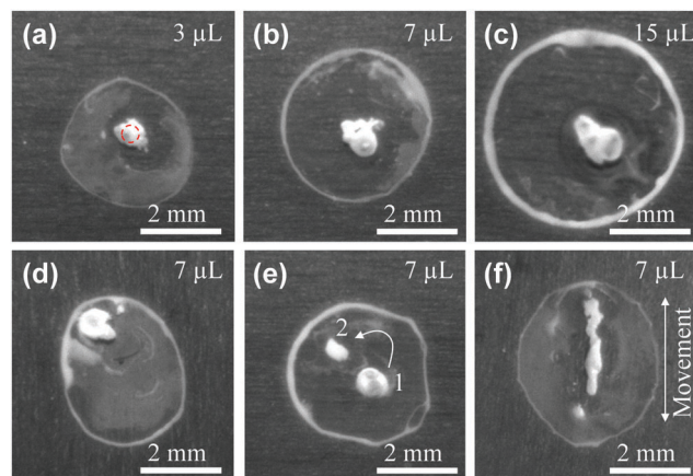
Fig. 4 Pattern formation for PS nanoparticles under laser irradiation under various conditions. (a–c) Laser spot in the central region of the droplet. (d) Laser spot located at the top left in the image of the droplet. (e) Laser spot at position 1 and then moved to position 2. (f) The substrate was moved relative to the laser beam with a constant speed of \sim 0.12 \text{ mm s}^{-1} . All droplets were irradiated with an \sim 0.43 mm-diameter laser spot, represented as a dashed circle in (a), and a power density of 151 \text{ W cm}^{-2} . The droplet volume is indicated in the top-right of each image.
