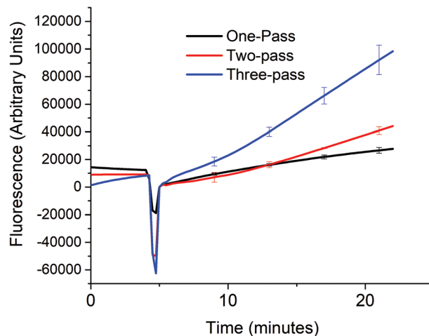
Fig. 3 Signal enhancement from multiple-pass target recycling. A 5 nM target DNA was added to a solution containing 50 nM of either only P 0 A 1 A 2 (one-pass), both P 0 A 1 A 2 and P 1 S (two-pass), or P 0 A 1 A 2 , P 1 S, and P 2 S (three-pass) and the reaction buffer mixture (1× NEBuffer 1 with 50 mM Mg 2+ ) and 20 μL 1 U μL -1 of exo III. The fluorescence signal was measured every 15 seconds at room temperature. (At t = ~5, the signal dropped because the spectrofluorometer was opened when exo III was added.)
