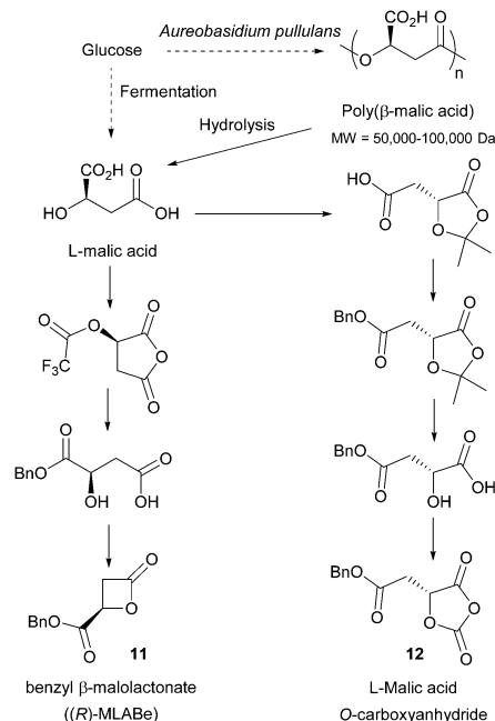
Fig. 9 Proposed pathway for the bioproduction of malic acid and conversion to 5-(S)-[(benzyloxycarbonyl)methyl]-1,3-dioxolane-2,4-dione (L-malOCA) monomer and to benzyl \beta -malolactonate.
