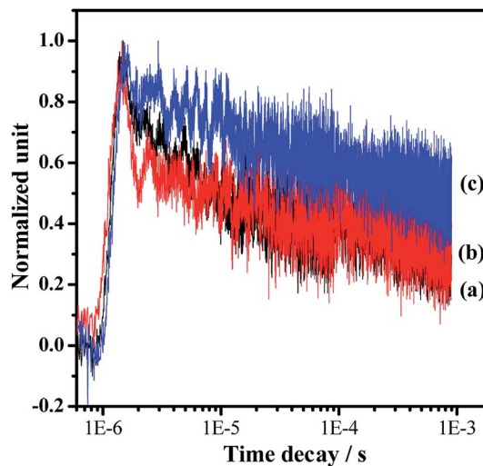
Fig. 6 Normalized transient absorption profiles of the representative samples in a vacuum: (a) Pt-Ta 3 N 5 , (b) Pt/Ba-Ta 3 N 5 and (c) Pt/Ba-Ta 3 N 5 . The pulse laser at 355 nm was used to excite the samples for the IR tests. The cocatalyst of Pt with a loading amount of 0.5 wt% was deposited by impregnation and a subsequent H 2 reduction method.
