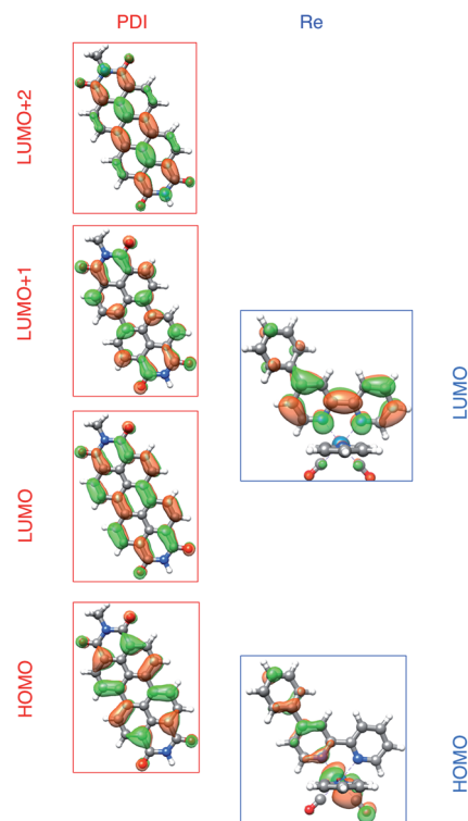
Fig. 7 Frontier molecular orbitals of PDI (left) and [\text{Re}(\text{Phbpy})(\text{CO})_3\text{-}(\text{py})]^+ molecular fragments calculated using DFT (isoval = 0.03). Frontier MOs of the full \text{PDI-}[\text{Re}(\text{Phbpy})(\text{CO})_3(\text{py})]^+ dyad are shown in Fig. S15.†
