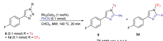
Scheme 5 Transannulation competition experiment revealing comparative reactivity of N -trifluoromethyl and N -tosyl triazoles with benzonitrile.
