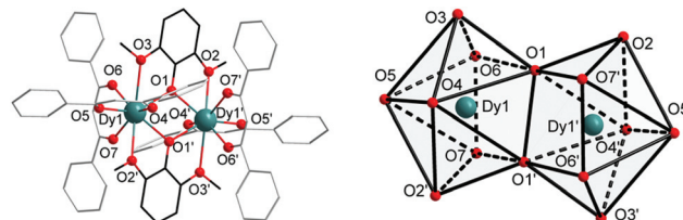
Fig. 1 Molecular structure of complex 1 with atomic labelling, in which a symmetry code was used to generate equivalent atoms: Dy' and O' (left), and the biaugmented trigonal prism of the [\text{DyO}_8] cores (right), hydrogen atoms have been omitted for clarity; symmetry codes: Dy1': 1 - x, -y, -z + 1 .
