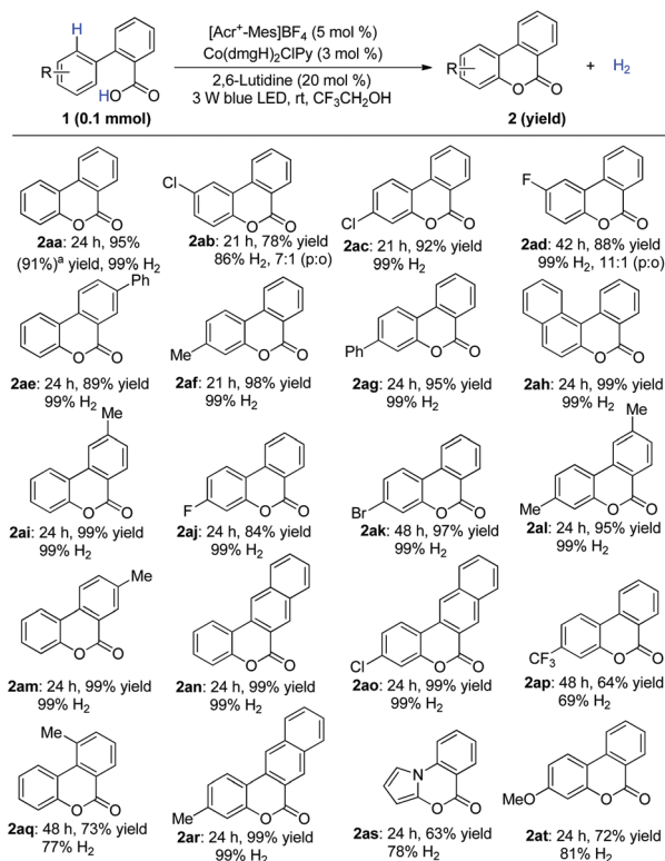
Scheme 2 Scope of substituted 2-arylcoumarins. a 8 mmol scale, [Acr + -Mes]BF 4 (3 mol%), Co(dmgH) 2 ClPy (1.5 mol%) and 2,6-lutidine (20 mol%) under 30 W blue LED.
