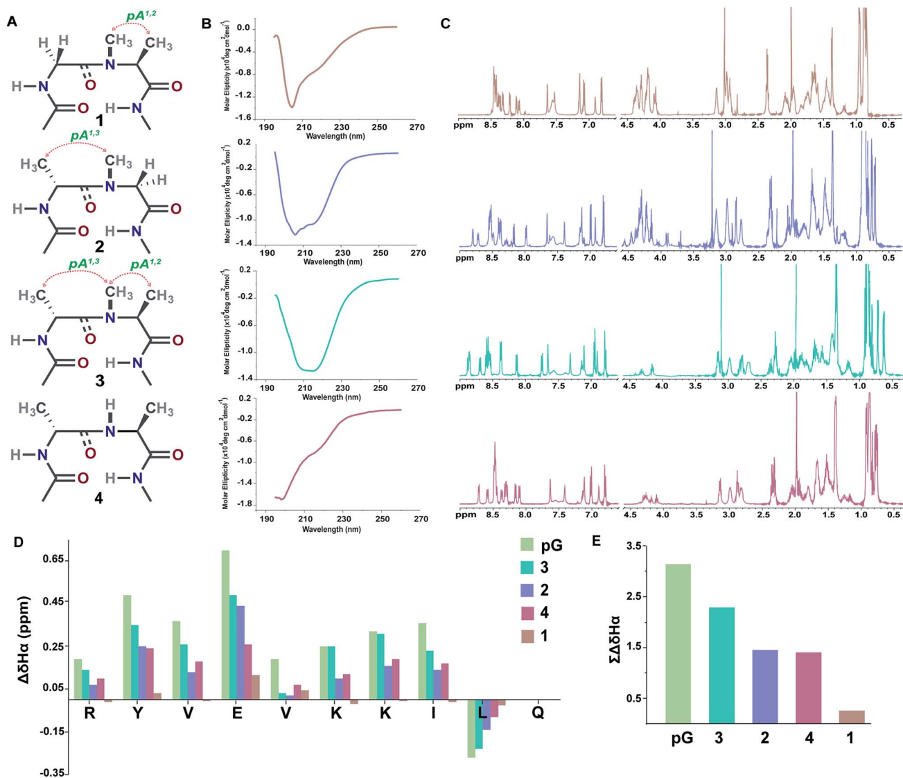
Fig. 3 (A) Interplay of pseudoallylic strain ( pA^{1,2} and pA^{1,3} ) in the reverse turn to induce the \beta -sheet folding. Note the spatial positioning of the methyl groups between i+1 \text{C}^\alpha and i+2 \text{C}^\alpha which modulates the folding of the polypeptide in aqueous solution at 25 °C. (B) CD spectrum of the peptides in acetate buffer (pH 3.8). (C) ^1\text{H} NMR in acetate buffer (pH 3.8), clearly indicating the enhanced dispersion of the \text{H}^N resonance and upfield shifted, distinguishable Leu11 \text{H}^{\delta 1/2} in the well-folded peptides. (D) Secondary chemical shifts obtained from the respective random coil control peptides, where the D-residue is substituted with the L-residue. Leu11 \text{H}^\alpha shows a negative deviation due to its proximity to the phenyl ring of Tyr2 in the folded analogs. In 1, the secondary chemical shifts were determined by subtracting the \text{H}^\alpha chemical shifts from the mean random coil chemical shifts of the respective residues obtained from the random coils of 2 and 3. The ring constrained reverse turn motif, pG, was taken as a reference. 19 (E) Summation of the secondary chemical shifts; only the absolute values were considered.
