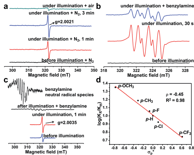
Fig. 1 (a) ESR detection of the electron transfer process in PCN-222. (b) ESR detection of O_2^{\cdot-} generation over PCN-222 trapped by DMPO. (c) The detection of hole-involved intermediates in PCN-222. (d) Hammett plot for the oxidation of benzylamine and its para -substituted derivatives photocatalyzed by PCN-222. All ESR tests were described in detail in the Experimental section.
