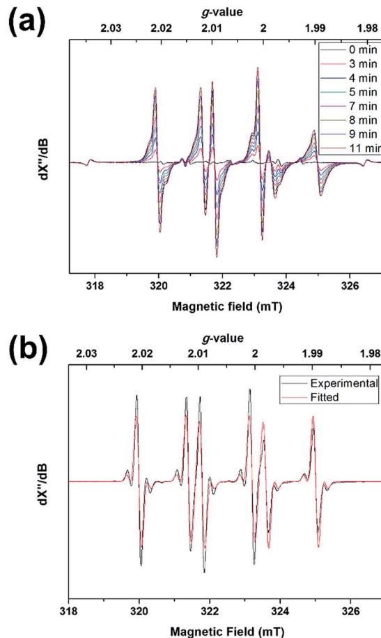
Fig. 7 Spin trapping of 2 . (a) EPR monitoring of a toluene solution of 1 and PBN at -50\text{ }^{\circ}\text{C} , under visible light irradiation (Xe lamp, 420–780 nm), and (b) fitting of the EPR spectrum of the same sample, recorded at -20\text{ }^{\circ}\text{C} .
