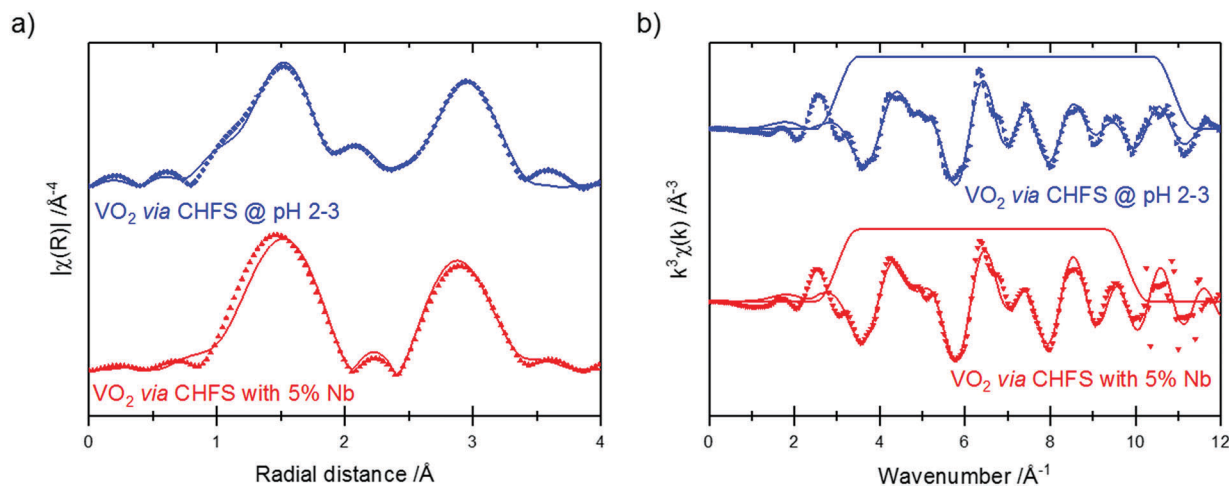
Fig. 7 V K-edge Fourier transforms (a) and EXAFS (b) of the CHFS VO 2 samples. Data are plotted as symbols, and fits as solid lines. The trapezoid lines in (b) indicate the Fourier transform window used.
