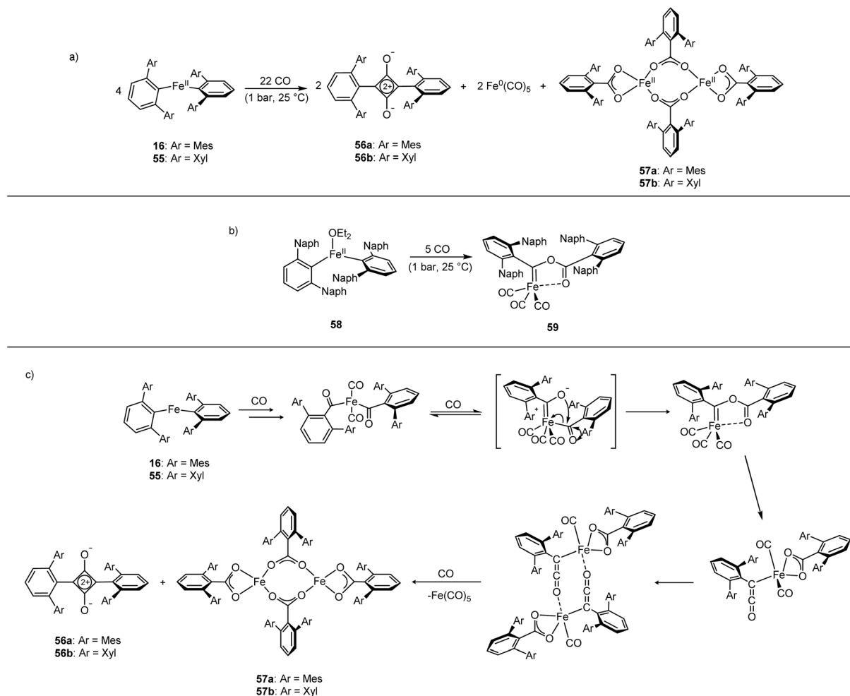
Scheme 23 Reactions of Fe(II) m -terphenyl complexes with CO. (a) Mes and Xyl substituted compounds ( 16 and 55 ) react to give squaraines ( 56a – b ), iron carboxylates ( 57a – b ), and Fe(CO) 5 . (b) Naphthyl substituted 58 reacts with CO to afford iron-carbene 59 . (c) Proposed mechanism for the reaction between 16 or 55 with CO. 132
