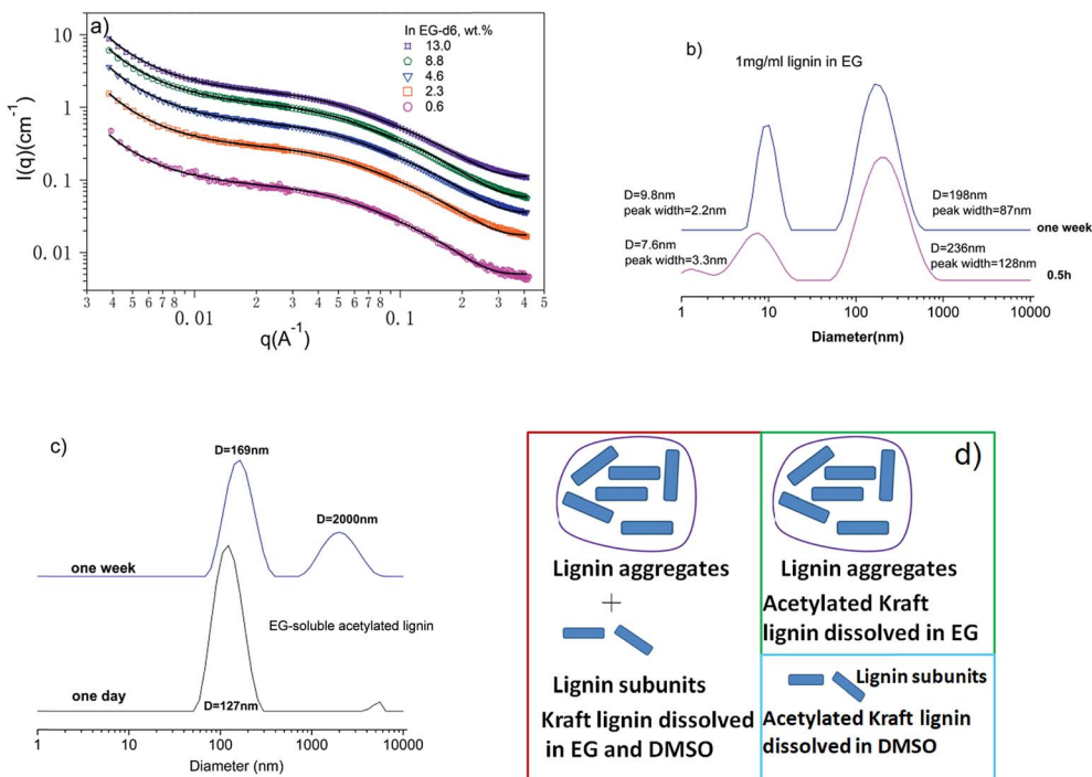
Fig. 1 (a) SANS data of lignin in EG with different concentrations. The solid lines are a fit to eqn (1). (b) DLS data of 1 mg ml -1 lignin in EG. (c) DLS data of dissolved acetylated lignin in EG. (d) Schematic illustrations of the solution structures of lignin and acetylated lignin in EG and DMSO.
