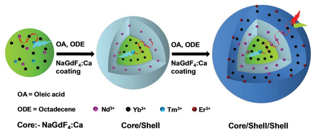
Scheme 1 Schematic illustration of the synthesis of CSS UCNPs following a seed-mediated layer-by-layer growth method.
