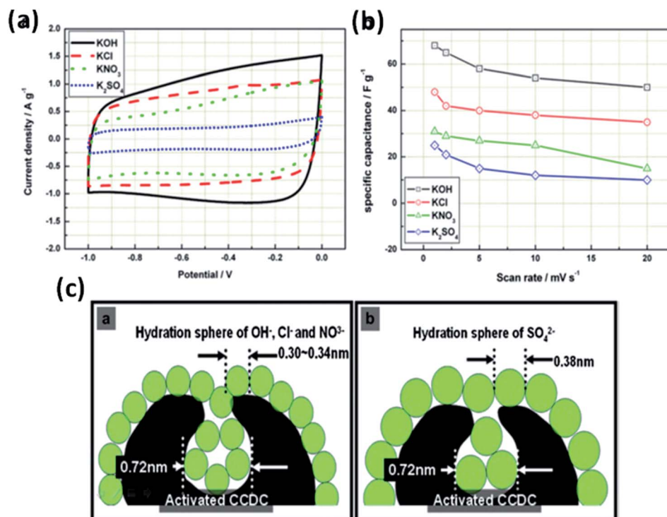
Fig. 8 (a) Cyclic voltammograms of activated CCDC supercapacitors in the aqueous electrolytes 0.5 M K_2SO_4 , 2 M KCl, 1 M KNO_3 and 6 M KOH ( 20 \text{ mV s}^{-1} ) and (b) the specific capacitance of the supercapacitor at different scan rates. (c) Schematic diagram of the relationship of hydration sphere ions and pores. This figure has been adapted from ref. 115 with permission from Elsevier.
