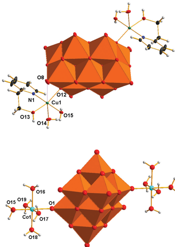
Fig. 1 Molecular structures of the anions [\{Cu(H_2O)_2(2\text{-hep})\}_2V_{10}O_{28}]^{2-} ( V_{10}Cu ) and [\{Co(H_2O)_5\}_2V_{10}O_{28}]^{2-} ( V_{10}Co ) as revealed by X-ray crystallography showing atom labelling. Colour code: orange octahedra \{VO_6\} , green Cu, light blue Co, blue N, red O, black C, gray H. Ellipsoids are displayed at a 30% probability level.
