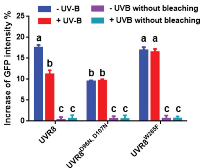
Fig. 4 Photobleaching results with the pFRET-NcCg-DEST vector. GFP fluorescence intensity was analysed before and after photobleaching for mCherry-UVR8-GFP, mCherry-UVR8 D96N,D107N -GFP and mCherry-UVR8 W285F -GFP expressed from the pFRET-NcCg-DEST vector (fusions abbreviated in the figure to UVR8, UVR8 D96N,D107N and UVR8 W285F ). Plants were exposed (+UV-B) or not (-UV-B) to 3 \mu\text{mol m}^{-2} \text{s}^{-1} broadband UV-B for 1 hour before being used for experiments. Primary data obtained as described in Fig. 3 are shown in Fig. S3,† together with the negative control results. The percentage increase in GFP fluorescence intensity after photobleaching for each construct was calculated by [(I_{\text{pb}} - I_{\text{pre}})/I_{\text{pre}}] \times 100 , where I_{\text{pre}} and I_{\text{pb}} indicate GFP intensities in the bleaching area before and after photobleaching, respectively. Means with S.E. are shown ( n > 5 ). Significance at P < 0.01 is indicated by letters.
