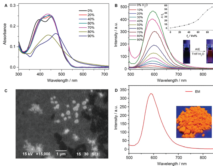
Fig. 2 Absorption and emission spectra: (A) absorption and (B) emission spectra of the AIEgen monomer EM (10 μM) in H 2 O/THF mixtures with different water fraction ( f_w ) from 0–90%, \lambda_{ex} = 460 nm; insets (B): plot of relative emission intensity against f_w and fluorescent images of EM ( f_w = 0 and 90%) under UV light illumination. (C) SEM image of nanoaggregates obtained from the EM suspension ( f_w = 90%). (D) Emission spectrum of EM in the solid state, \lambda_{ex} = 460 nm; inset: fluorescent image of the solid EM under UV light illumination.
