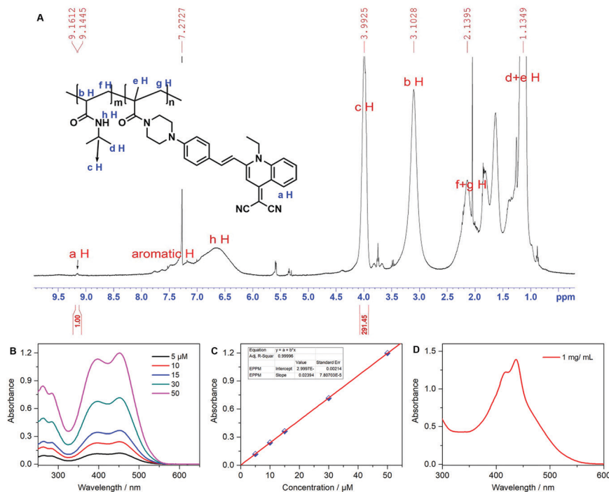
Fig. 1 Structure characterization of the fluorescent thermometer system: (A) 1 H NMR spectra of copolymer P(NIPAM-co-EM) in CDCl 3 . (B) Absorption spectra of the AIEgen monomer EM at different concentrations in THF (5–50 μM). (C) The corresponding standard working curve obtained from absorbance at 452 nm as a function of concentration. (D) Absorption spectrum of P(NIPAM-co-EM) in THF (1.0 mg mL -1 ).
