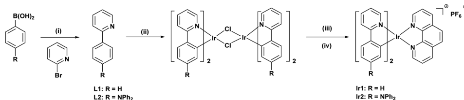
Scheme 1 Synthesis of cyclometalated Ir(III) complexes. (i) Pd(OAc) 2 , K 2 CO 3 , EtOH/H 2 O 3:1 (v/v), 80 °C in air, 30–60 min. (ii) IrCl 3 ·3H 2 O, EtOCH 2 CH 2 OH/H 2 O, 3:1 (v/v), 110 °C, N 2 , 24 h. (iii) 1,10-Phenanthroline, EtOCH 2 CH 2 OH, 120 °C, N 2 , 24 h. (iv) KPF 6 , RT, 3 h.
